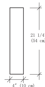
Side Splash / Bande anti-éclaboussure
